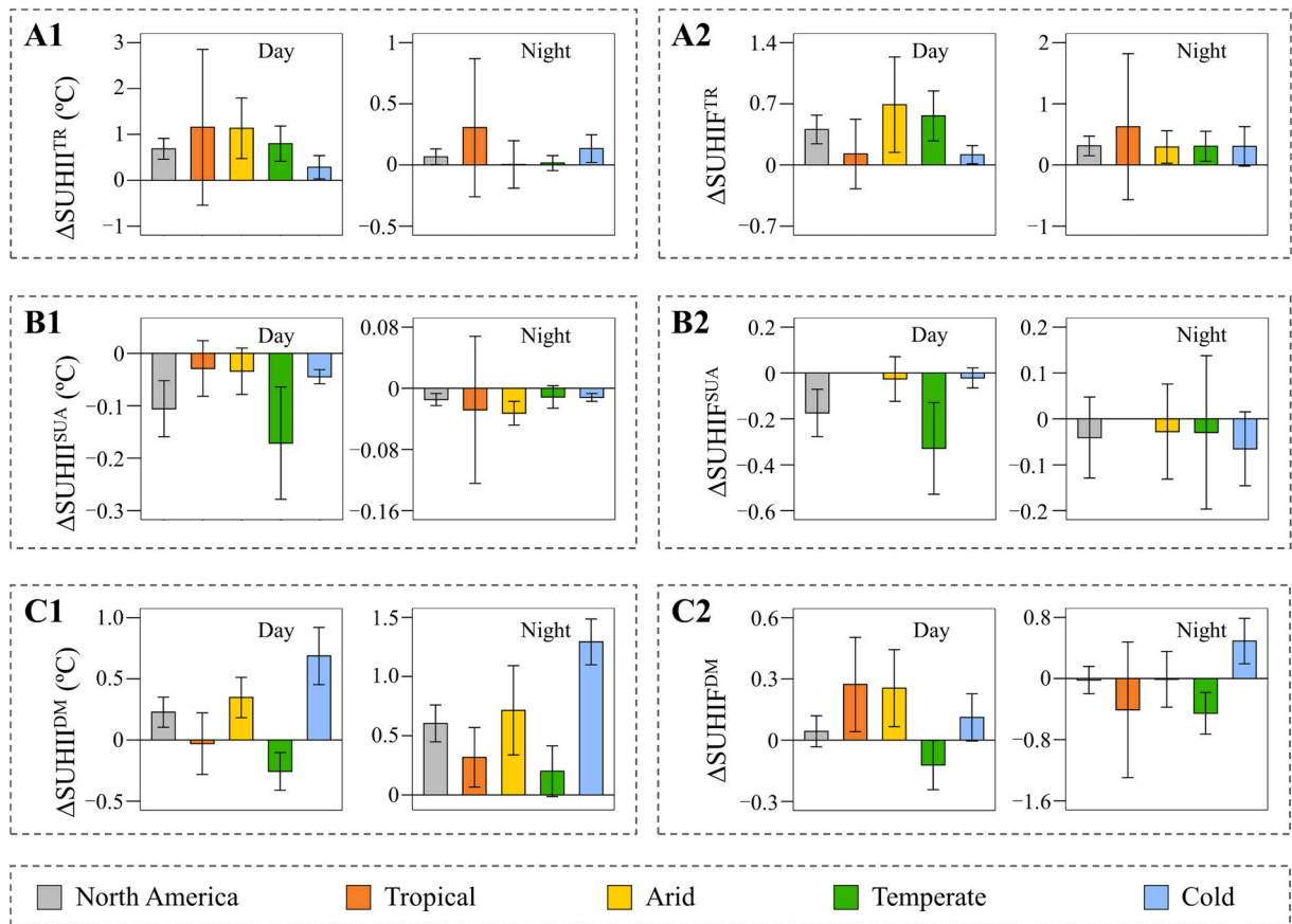
Fig. 10. Influence of confounding factors on the SUHI intensity (SUHI) and footprint (SUHIF) estimated by the ASE method. (A) The average difference in the SUHI ( \Delta\text{SUHI}^{\text{TR}} ) or SUHIF ( \Delta\text{SUHIF}^{\text{TR}} ) between that disturbed by topographic relief (TR) and that removed the influence of TR. (B) The average difference in the SUHI ( \Delta\text{SUHI}^{\text{SUA}} ) or SUHIF ( \Delta\text{SUHIF}^{\text{SUA}} ) between that disturbed by surrounding urban areas (SUAs) and that removed the influence of SUAs. (C) The average difference in the SUHI ( \Delta\text{SUHI}^{\text{DM}} ) or SUHIF ( \Delta\text{SUHIF}^{\text{DM}} ) between that estimated by the original MODIS LST data (disturbed by data missing (DM)) and that estimated by the gap-filled MODIS LST data. The histograms and bars represent the mean values and 95% confidence intervals, respectively.
