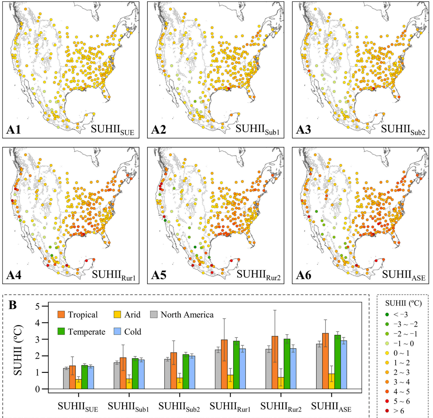
Fig. 5. Spatial contrast of the annual daytime SUHI intensity (SUHII) obtained by different methods. (A) Spatial variation of the annual daytime SUHII across 254 North American cities. (B) Mean ( \pm 95% confidence interval) of the annual daytime SUHII.
