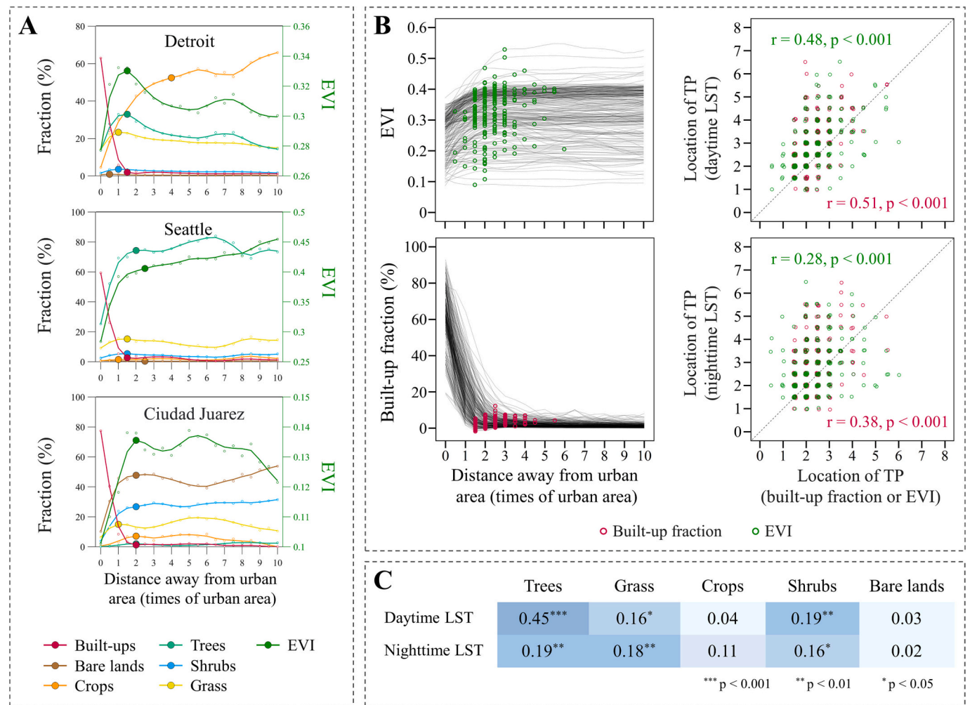
Fig. 17. Land cover changes along urban-rural gradients and their correlations with LST. (A) Changes in land cover fractions and the enhanced vegetation index (EVI) along urban-rural gradients and their turning points (TPs), taking 3 cities as examples. (B) The TPs of built-up fraction and EVI and their correlation with those of LST across all North American cities. (C) Pearson correlation coefficients of TPs between LST and the fraction of different land covers.
